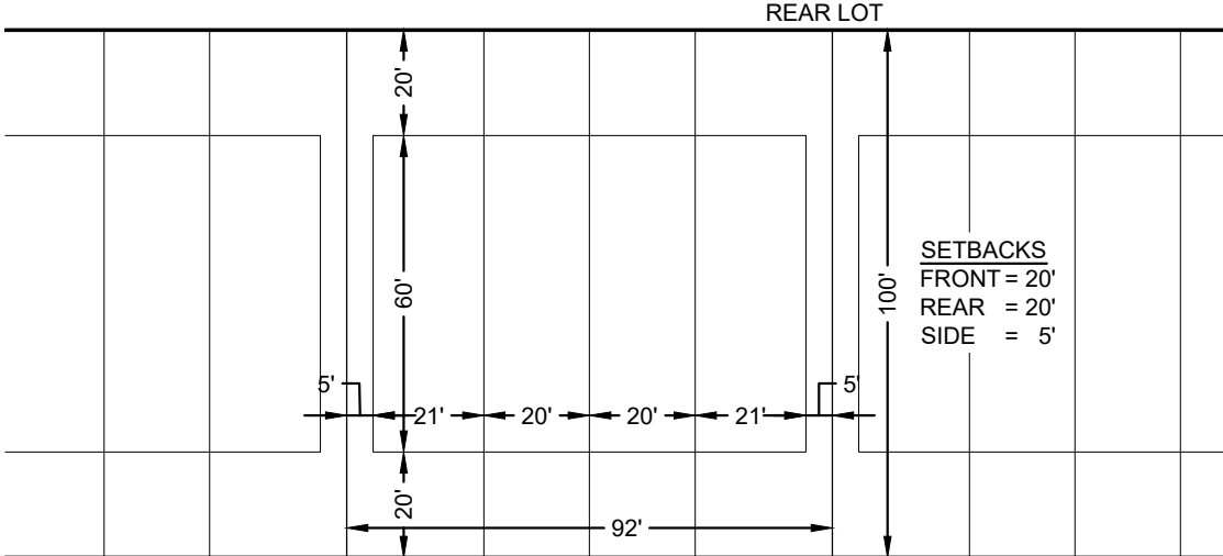
FRONT LOAD TOWNS (4-PLEX) LOT DETAIL
