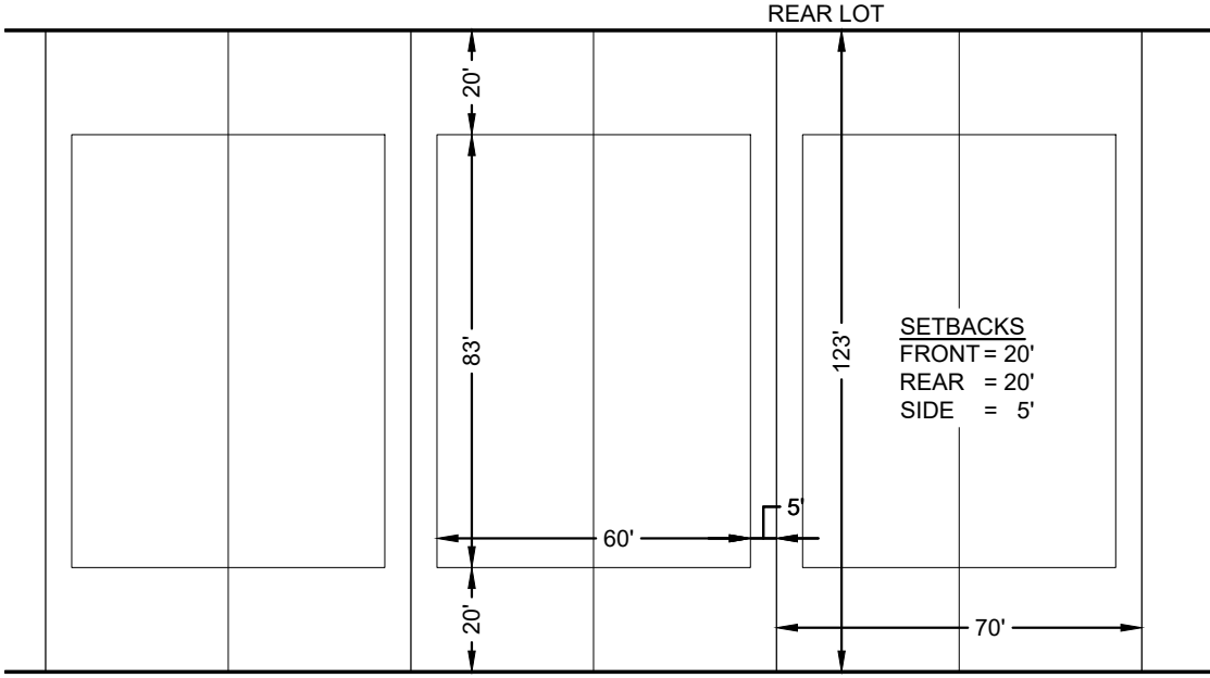
PAIRED VILLAS (DUPLEX) LOT DETAIL
