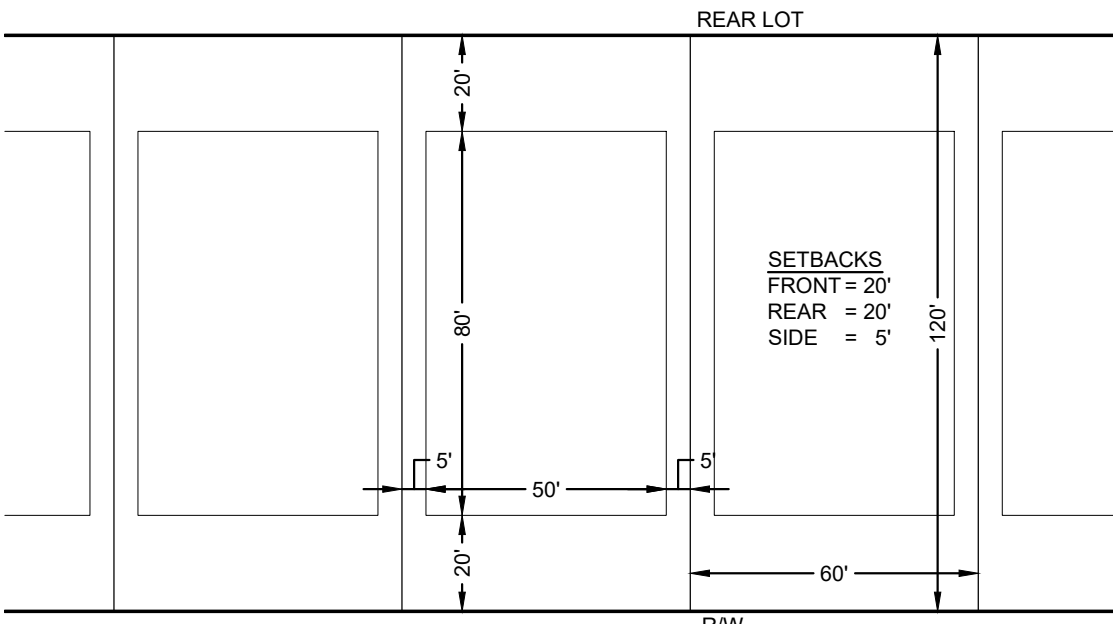
60' LOT DETAIL
