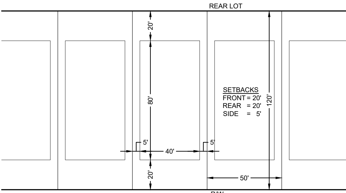
50' LOT DETAIL
