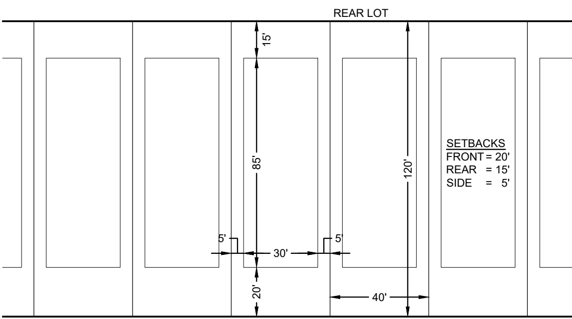
40' LOT DETAIL
